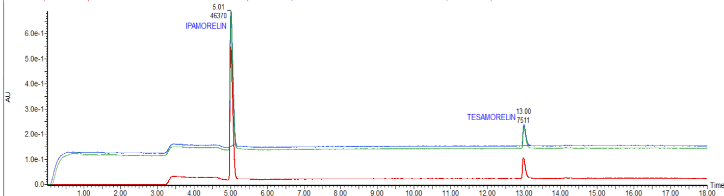
UV CHROMATOGRAM
