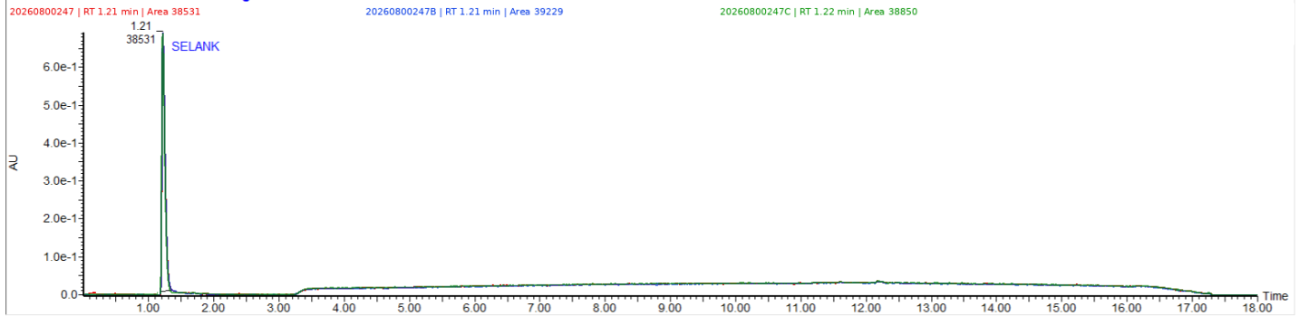
UV CHROMATOGRAM
