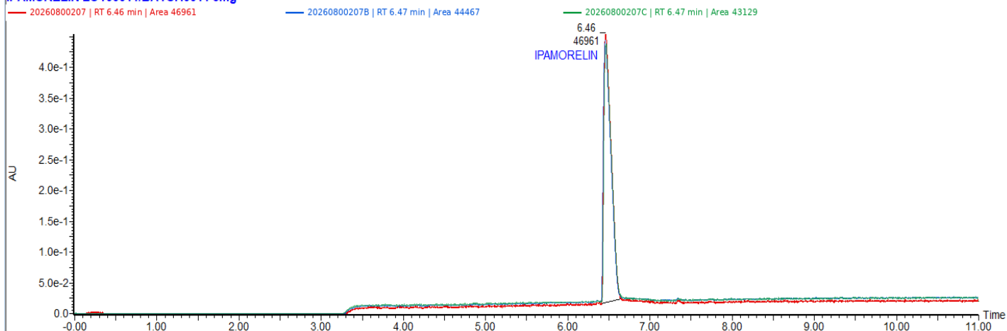
UV CHROMATOGRAM
